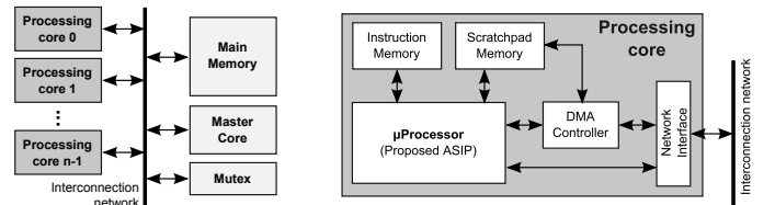
(a) General overview of the multi-core architecture.
