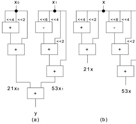
Fig. 2. Multiplierless realization of constant multiplications using the DBR technique [35]: (a) 21x_0 + 53x_1 ; (b) 21x and 53x .
