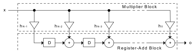
Figure 1: Transposed form FIR filter design.
