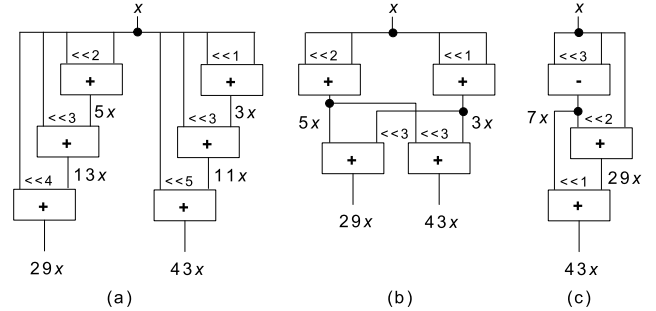
Figure 1. Solutions of the algorithms for the shift-adds implementation of constant multiplications 29x and 43x : (a) the digit-based recoding technique [3]; (b) the CSE method [4]; (c) the graph-based algorithm [5].
