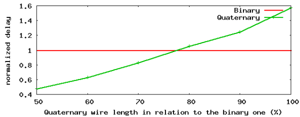
Fig. 3: Effects of wire lengths on the delay of the quaternary devices.
