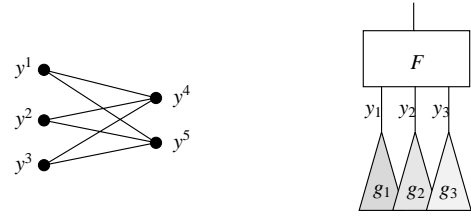
(a) Bipartite graph for F .
