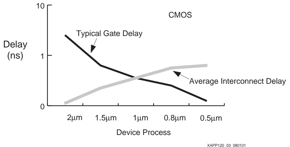
Figure 3: Importance of Interconnect vs Gate Delay
